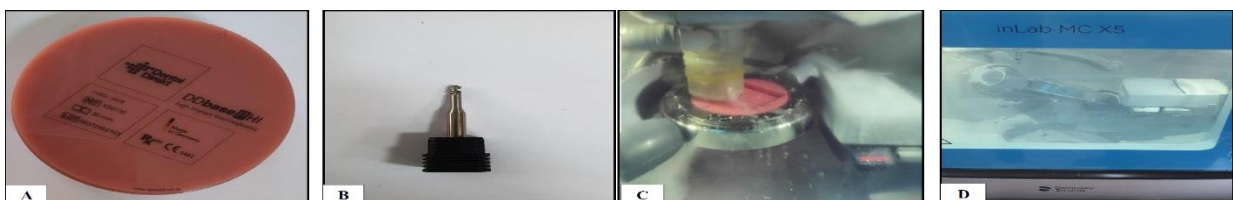
Fig. 2. (A) CAD/CAM block, (B) In Lab MC X5- miller for PMMA plastics, and (C, D) Dental milling machine MC X5 in lab
