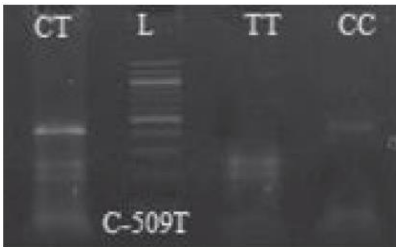
Fig. 1. TGFB1 C-509 T polymorphism representative gel photograph
